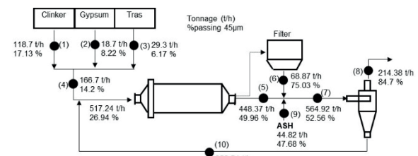
Figure 4. Mass balanced flowsheet of the sampled circuit in CEMI/42.5R Portland cement production (survey-1)
