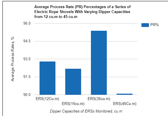
Figure 6. Process rates of the electric rope shovels monitored
