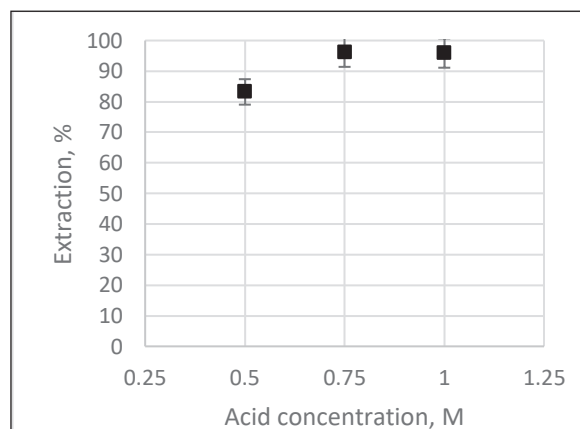
Figure 4. Effect of sulphuric acid concentration on extraction (Conditions: Temperature of 70°C, leaching time of 180 min, solid-to-liquid ratio of 1/10, stirring speed 400 rpm)
