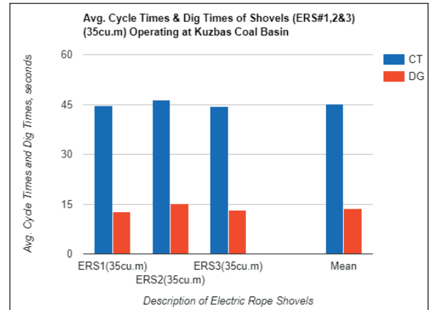
Figure 1. Average cycle and dig times of the electrical rope shovels
